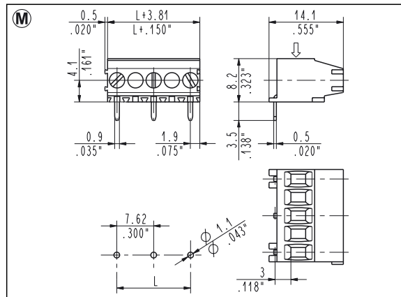
MTS_097 90°, Top Entry 7.62 mm / .300" Pitch Weight per pole: 0.94 g
